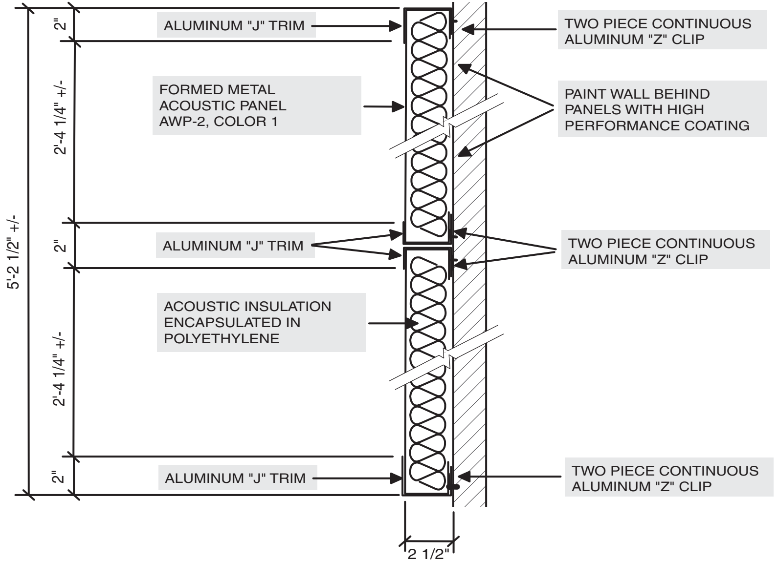
ACOUSTIC WALL PANEL MTG. DETAIL (W-01)
