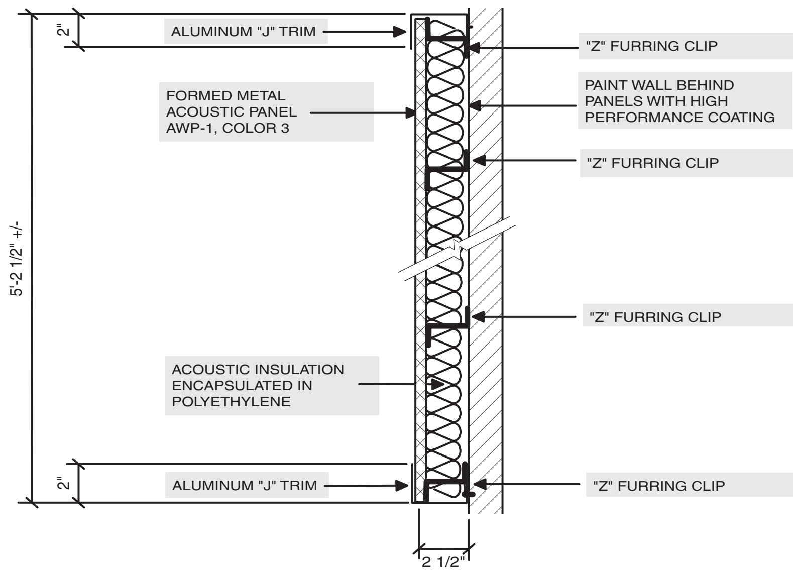
ACOUSTIC WALL PANEL MTG. DETAIL (W-02)
